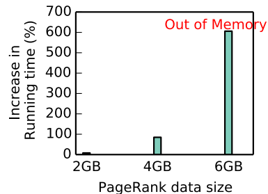
Figure 3. Simultaneous server revocations substantially increase running time if Spark runs out of available memory.
